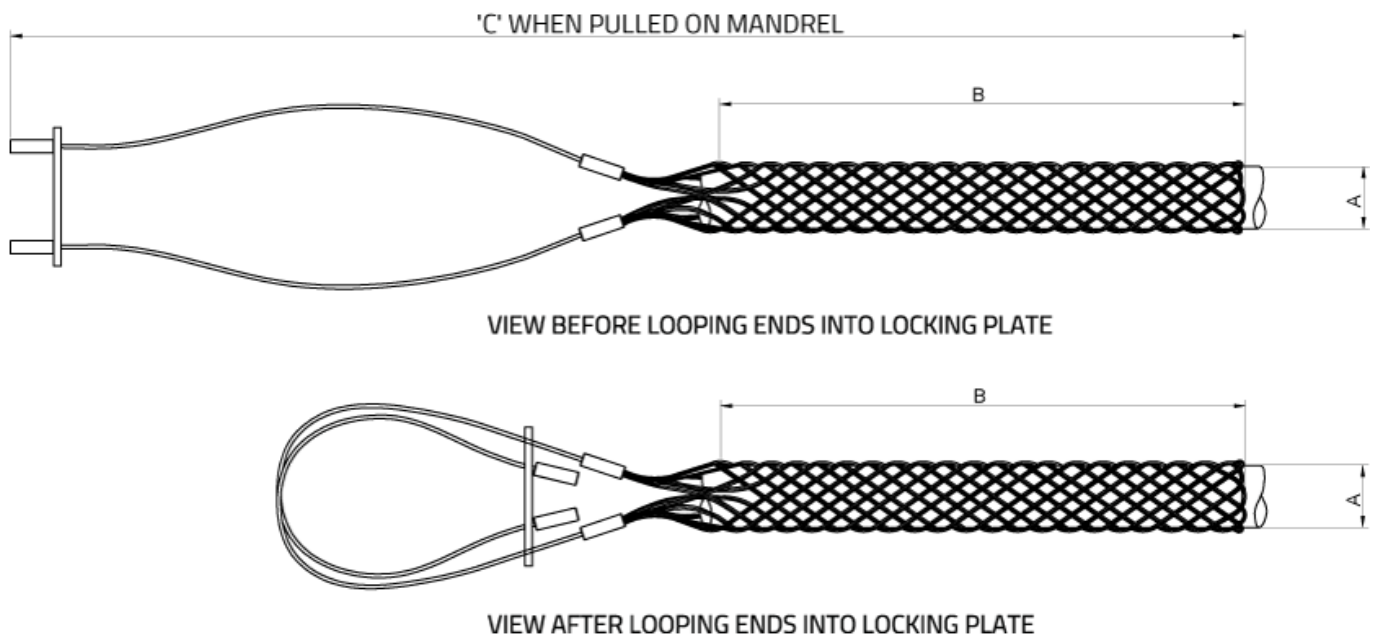
U Type Universal Eye Hose Sock - 316 Stainless Steel
